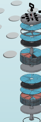
FILTER PACK WITH HIGH PROFILE DISCS
